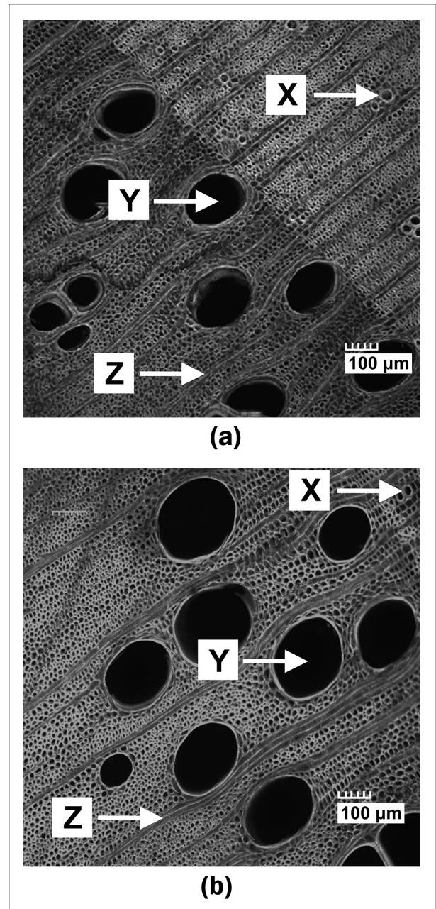
Figure 2. Transverse cross sections from a Fraxinus pennsylvanica , taken from tissues (a) discolored by trunk-injected emamectin benzoate and (b) unstained sapwood. The images were obtained using a confocal laser scanning microscope equipped with helium-neon ( \lambda = 543 nm) and argon ( \lambda = 488 nm) lasers. The three-dimensional images consists of (a) eight slices obtained 14.5 \mu m apart and (b) 27 slices obtained 10.3 \mu m apart. A 10 \times dry objective was used for magnification. Images show (X) latewood xylem vessels, (Y) earlywood xylem vessels, and (Z) xylem ray cells.
