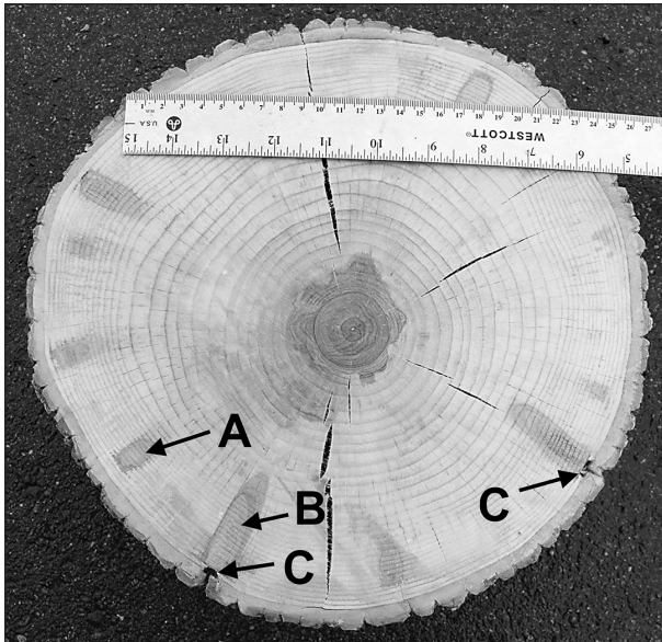
Figure 1. A cross section from a Fraxinus pennsylvanica tree, injected in May 2008 and 2009 with a low rate (0.1g a.i. per 2.54 cm at diameter at breast height) of emamectin benzoate (TREE-äge) applied with a QUIK-jet system. The cross section was cut 10 cm above 2008 injection sites. Discoloration from (A) 2008 and (B) 2009 injections and (C) 2009 injection sites are visible. Latewood is visible on the periphery of the 2009 injection sites. Cracking in the sapwood was caused by drying. Dark heartwood is present in the center for the cross section.
